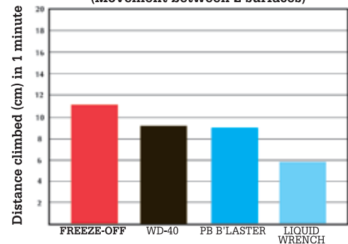
Capillary Penetration Test (Movement between 2 surfaces)
